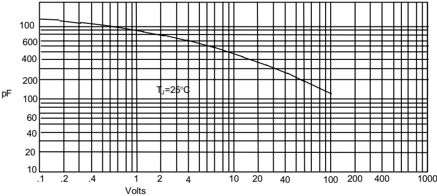
Figure 3 Junction Capacitance
